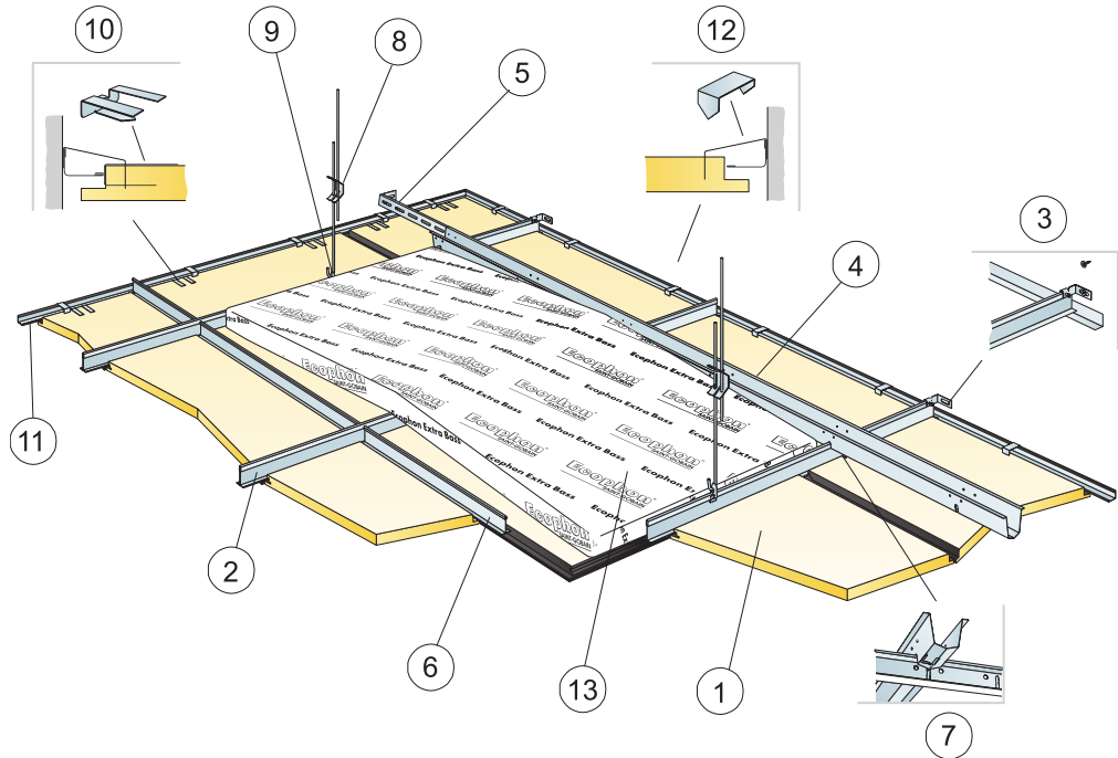
©Saint-Gobain Ecophon AB Installation diagram (M614) for Ecophon Focus Ds. Suspended installation
